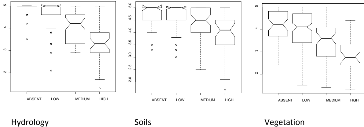
FIGURE C7. Notched Boxplot of MEF Ratings (x axis) within Condition in relation to Human Stressor Index (y-axis).
